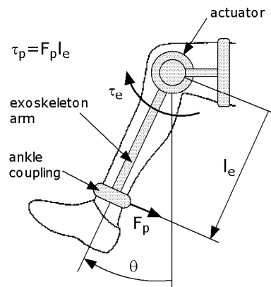
Fig. 1. Hypothetical 1-DOF exoskeleton.
